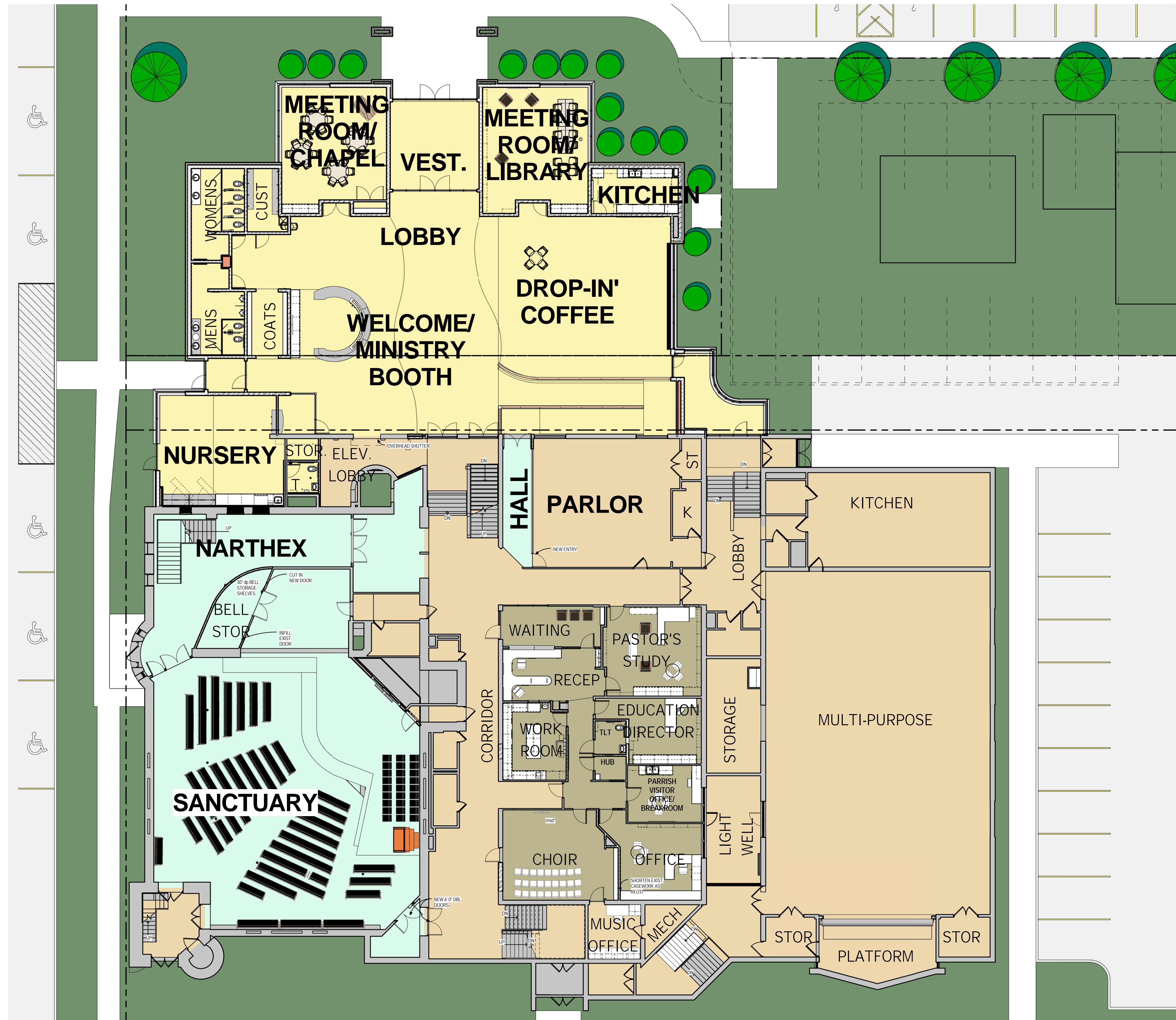
1 COLORED FULL PLAN DD-41 SCALE: 1" = 10'-0"
