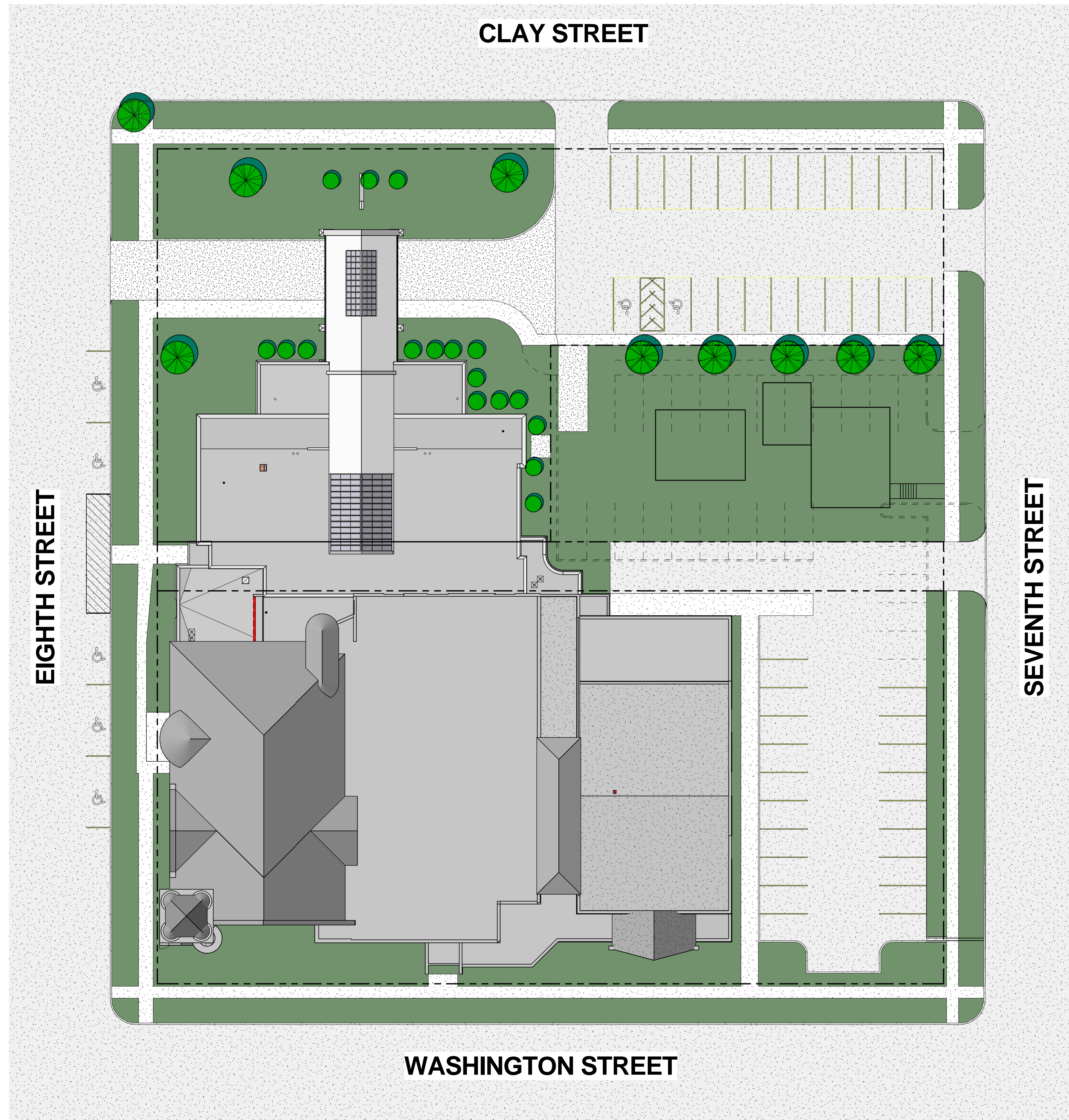
1 COLORED SITE PLAN DD-1 SCALE: 1/16" = 1'-0"
